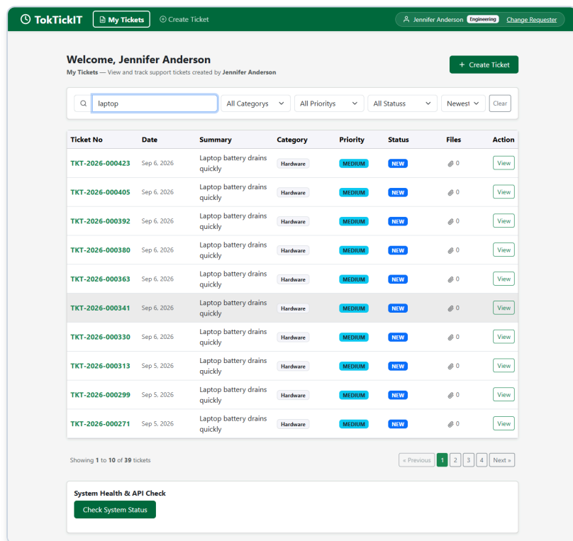
Filter Dropdowns
