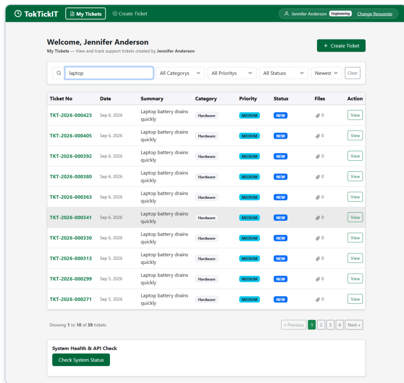
Search Feature
