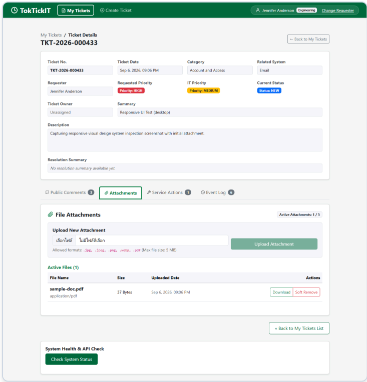
Download Attachment
