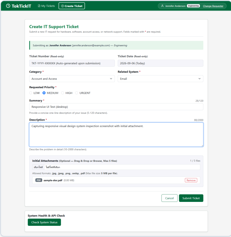
Desktop Viewport
