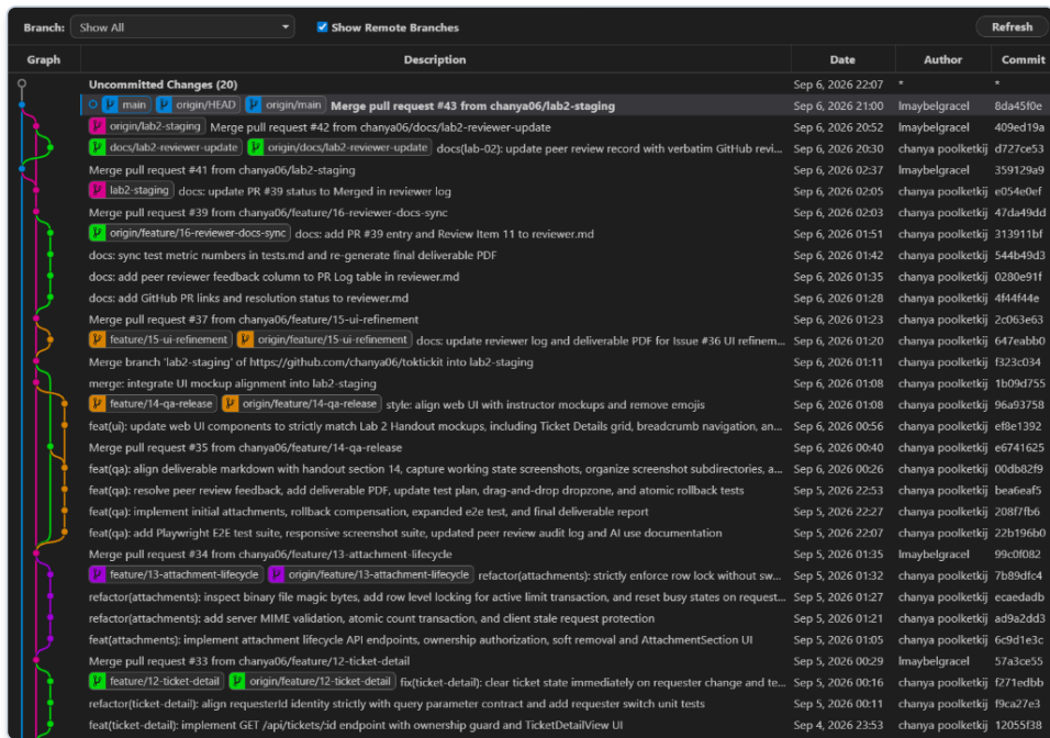
Git Commit Graph History Part 1
