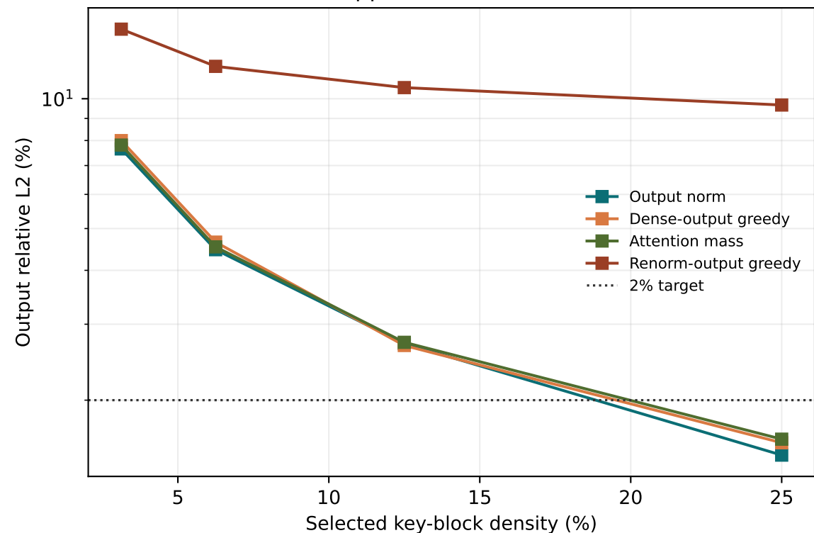
Normalization tax (best renorm-oriented router)
