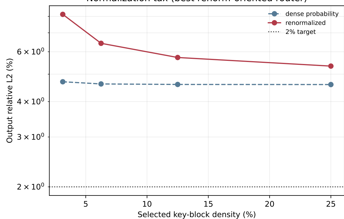
Normalization tax (best renorm-oriented router)
