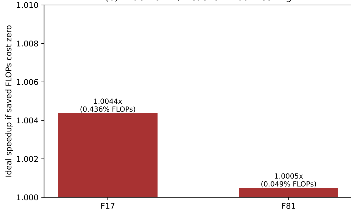
(b) Exact text K/V cache Amdahl ceiling
