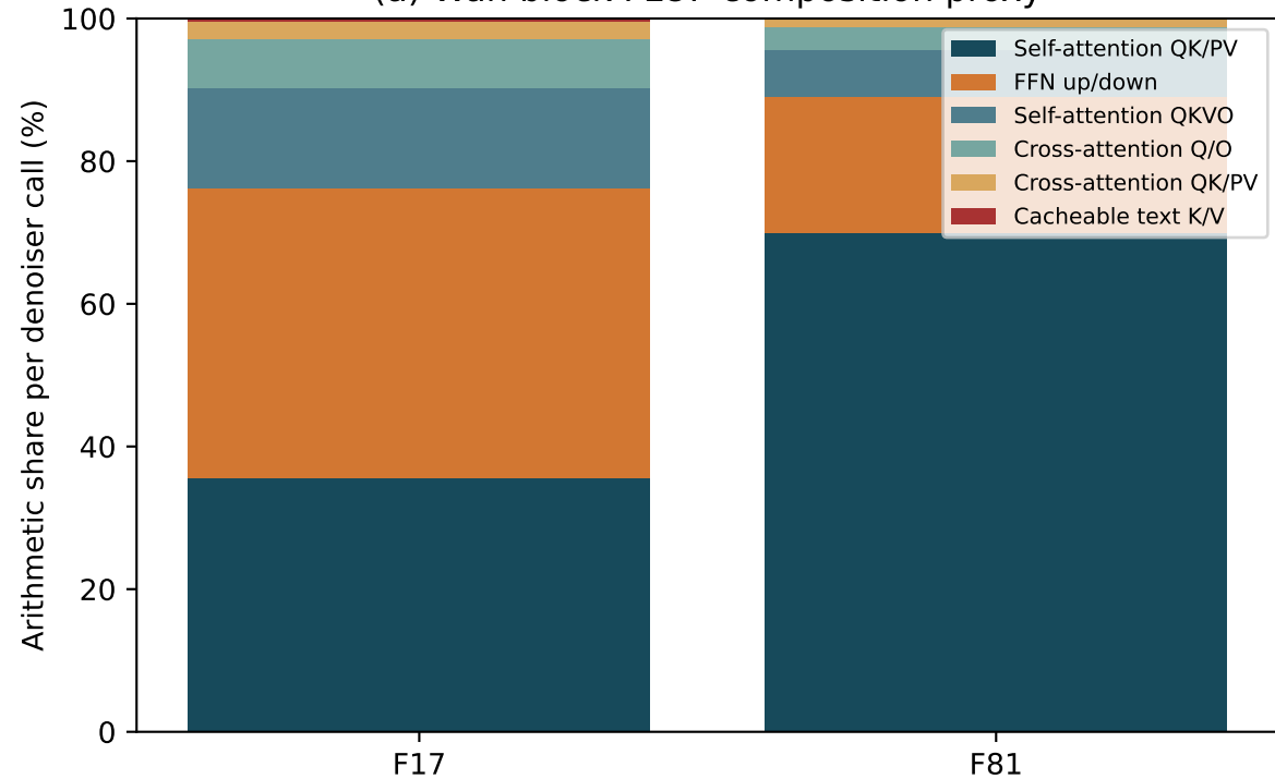
(a) Wan block FLOP composition proxy
