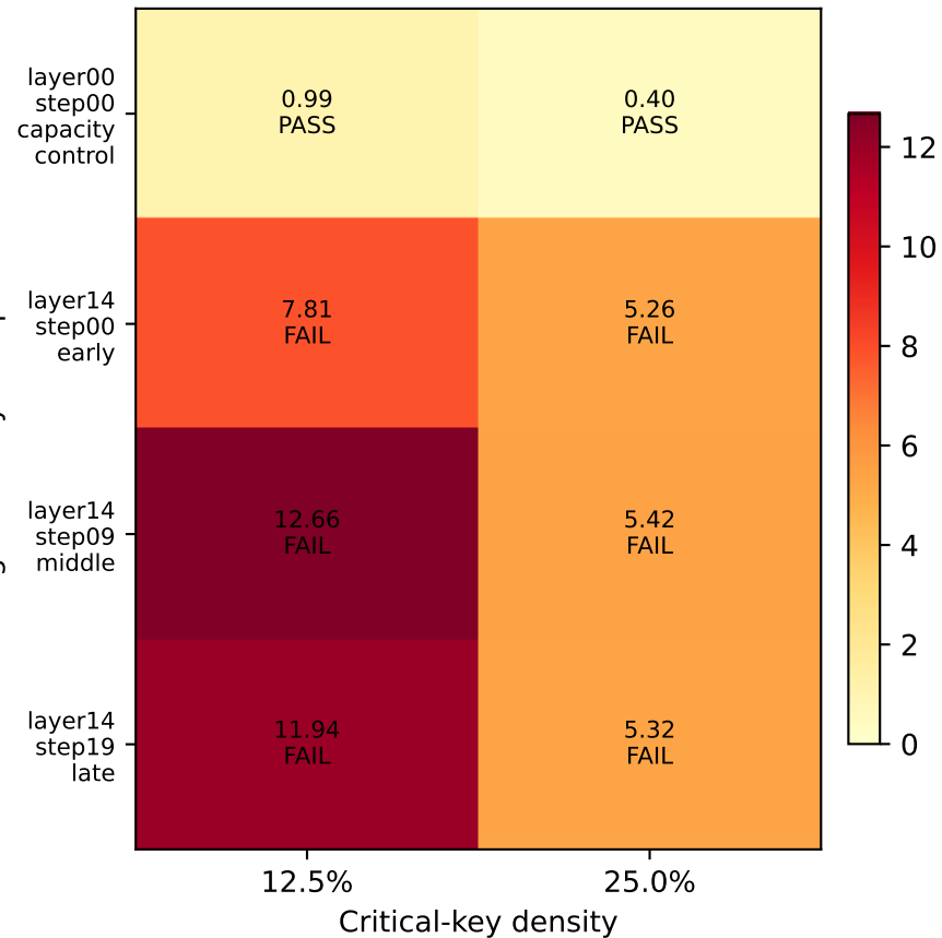
Worst record output error (%)
