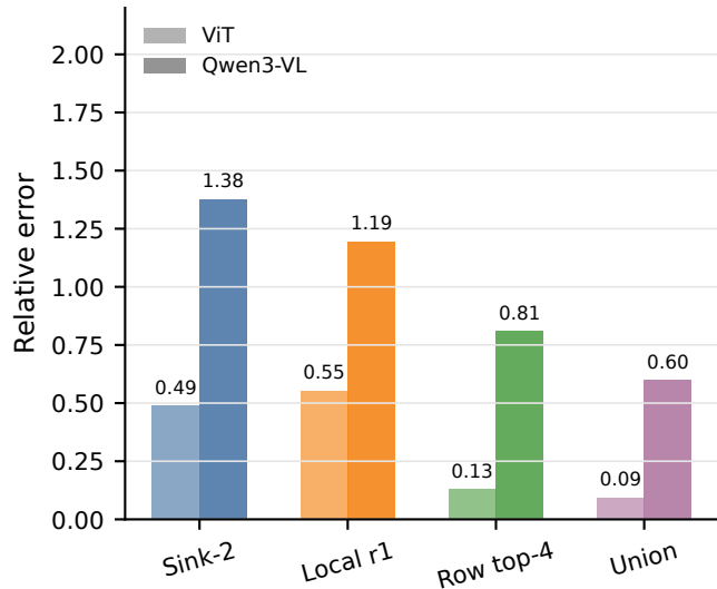
Keep-only A@V error
