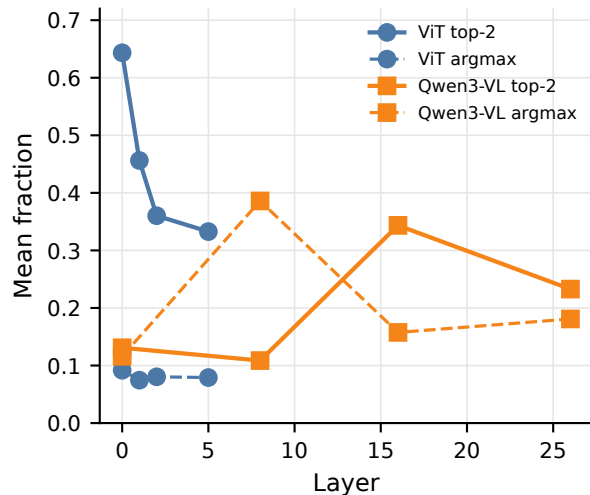
Sink / collapse by layer
