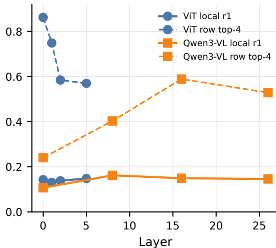
Local vs row-sparse mass
