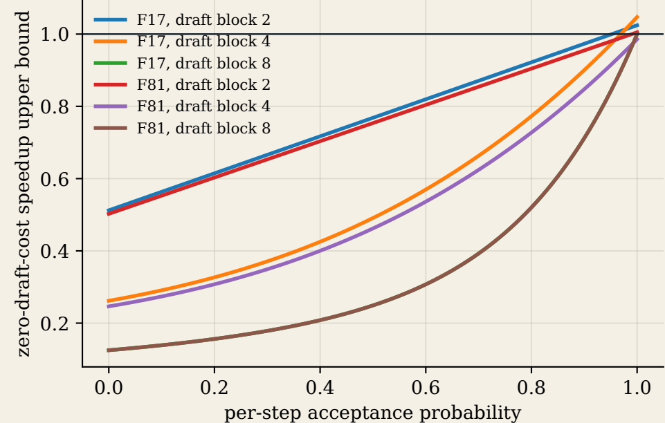
D Speculation needs sublinear verification
