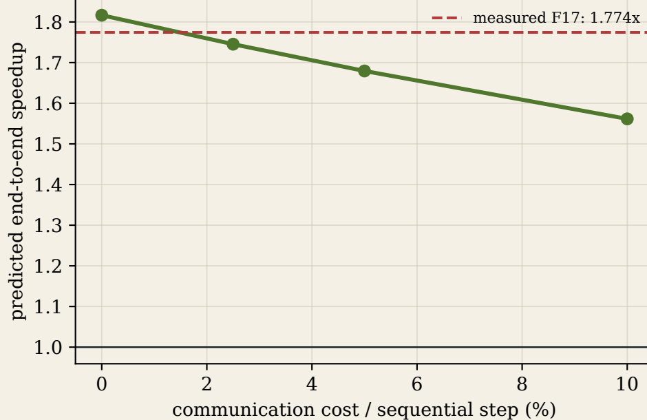
B Exact CFG optimistic envelope
