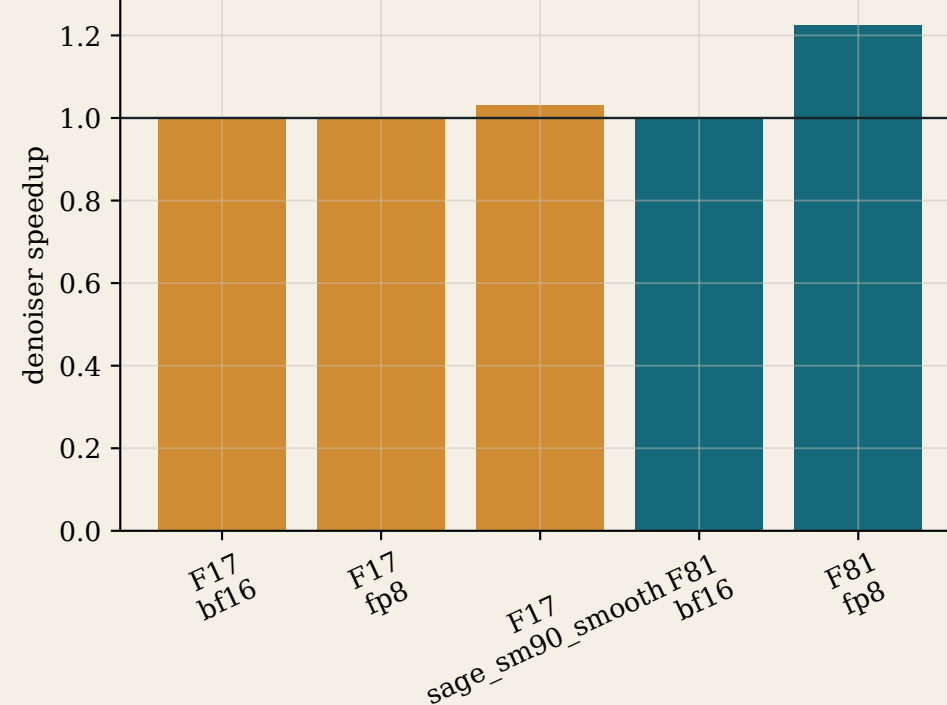
F Kernel gain is Amdahl-limited
