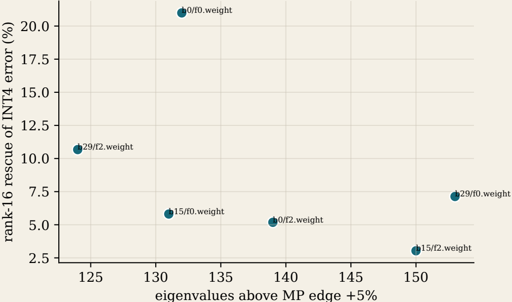
G MP spikes are signal, not a speed guarantee
