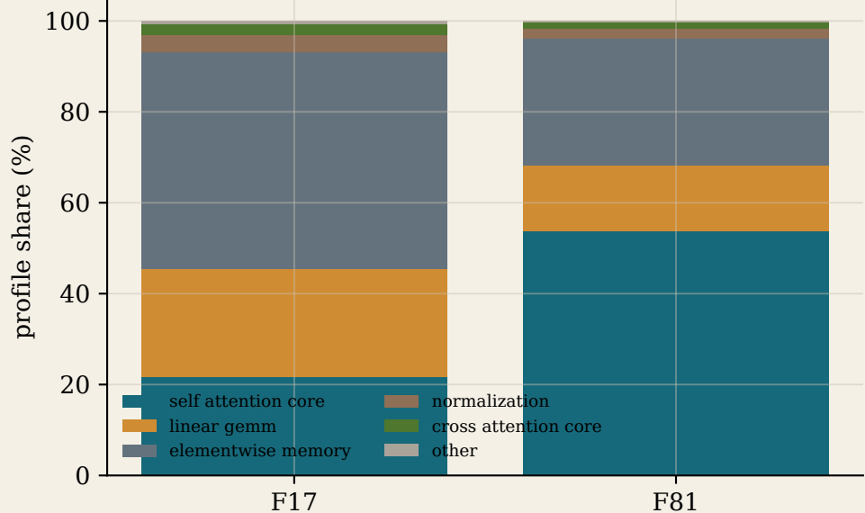
A Runtime bottleneck shifts with video length
