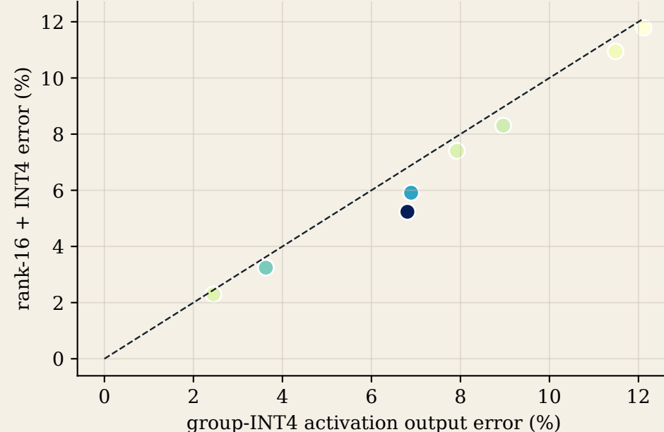
H Spectral tail helps but remains lossy
