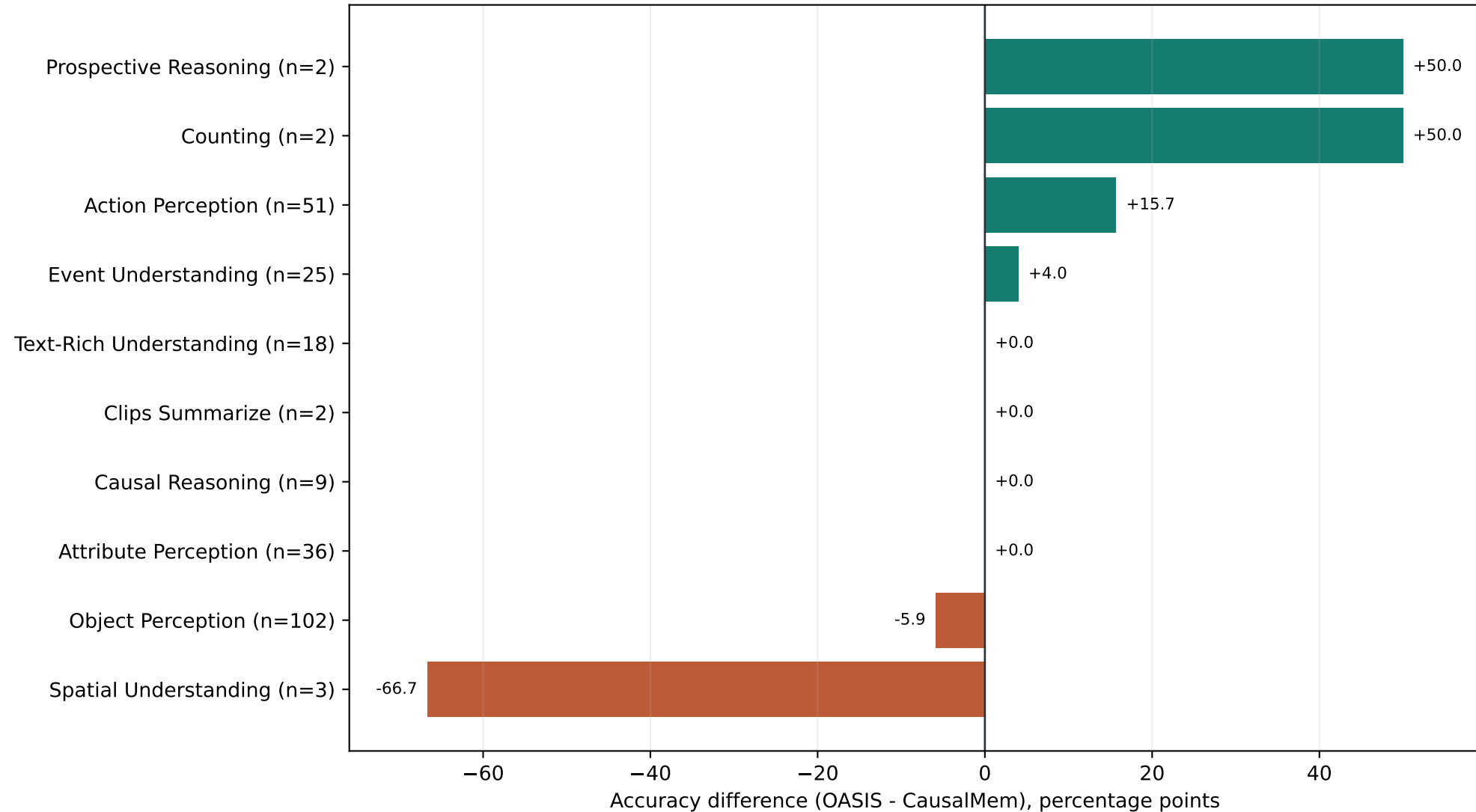
Paired task differences on StreamingBench RTU 1-50
