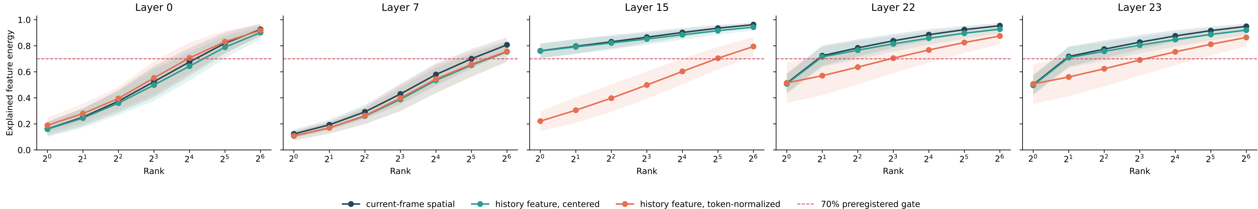
LLaVA-CLIP-ViT-L-336 persistent-state spectrum across analyzed segments
