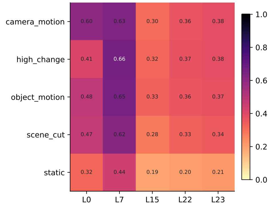
Local BTTB improvement vs identity (gate 0.10)
