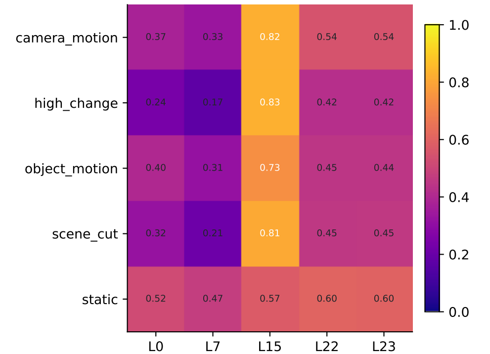
Local BCCB improvement vs identity (gate 0.10)
