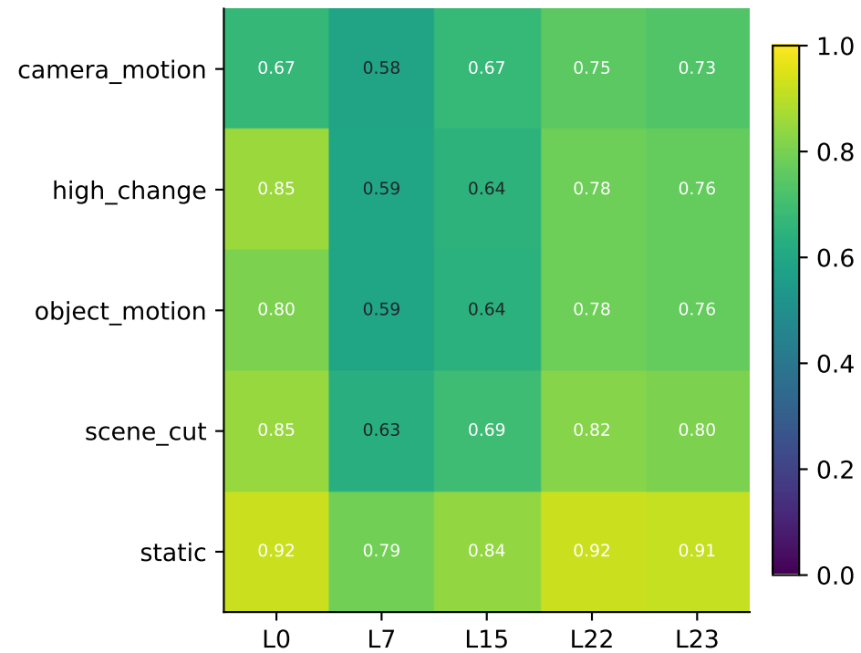
Optical-flow improvement vs identity (gate 0.10)
