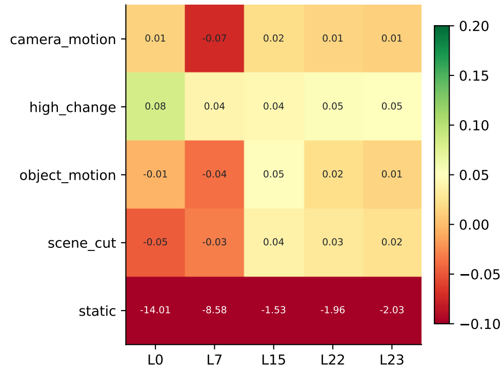
Optical-flow improvement vs identity (gate 0.10)
