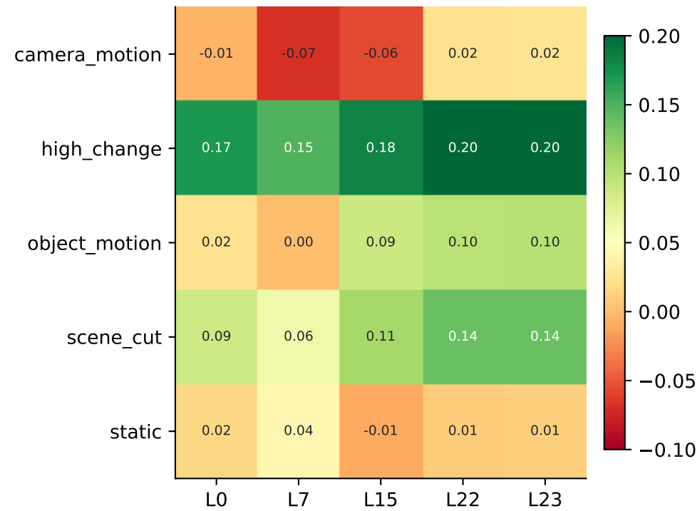
Local BTTB improvement vs identity (gate 0.10)
