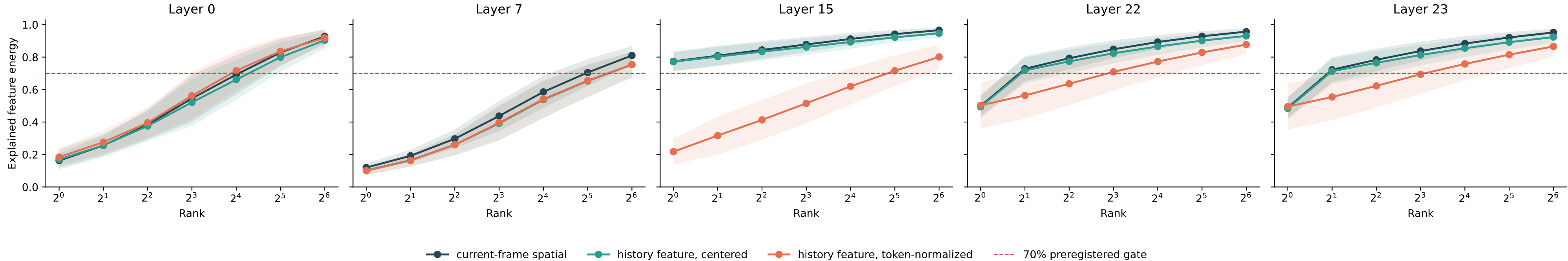
LLaVA-CLIP-ViT-L-336 persistent-state spectrum across three clips
