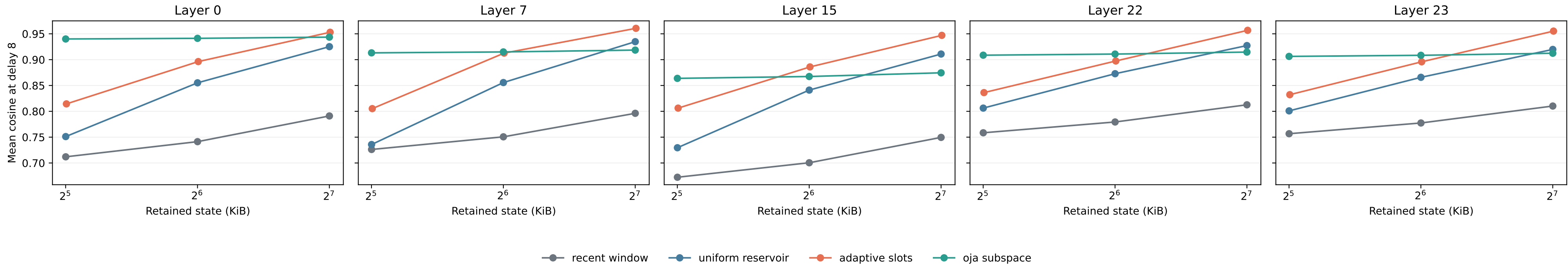
Matched-byte memory frontier
