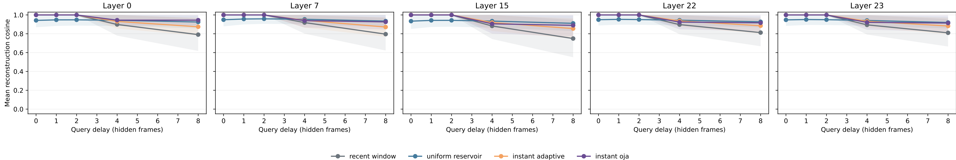
Matched-payload retention, capacity=64, mode=frame_centered_unit
