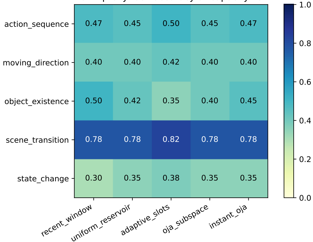
CLIP proxy task accuracy at capacity=8
