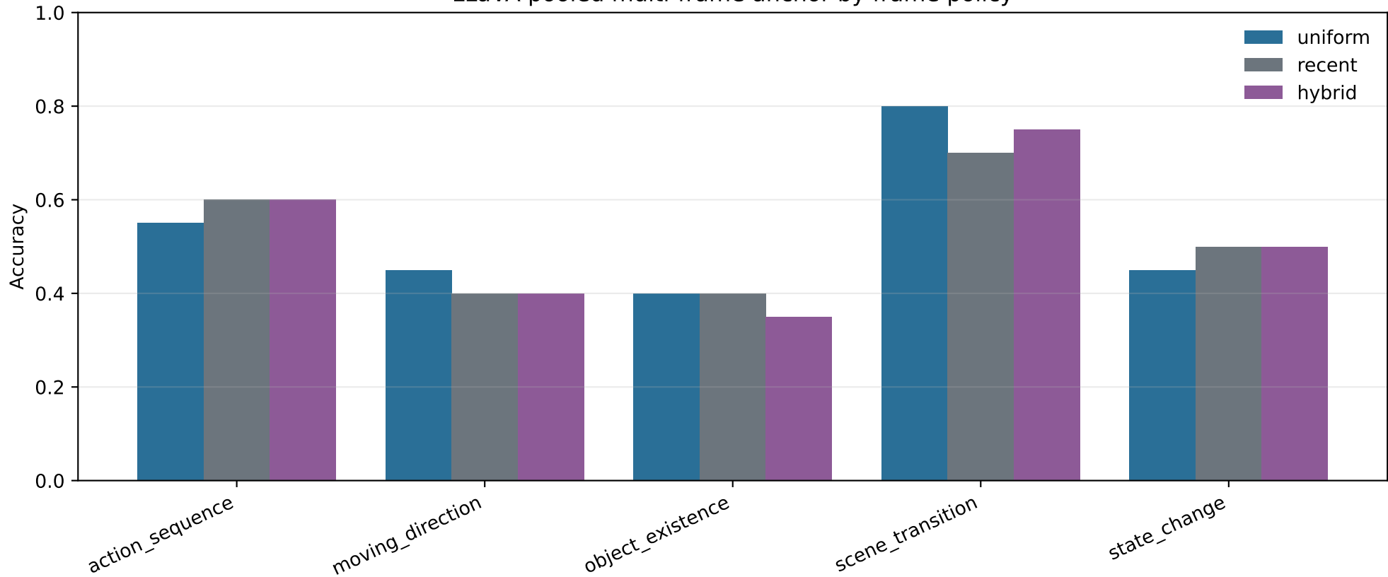
LLaVA pooled multi-frame anchor by frame policy
