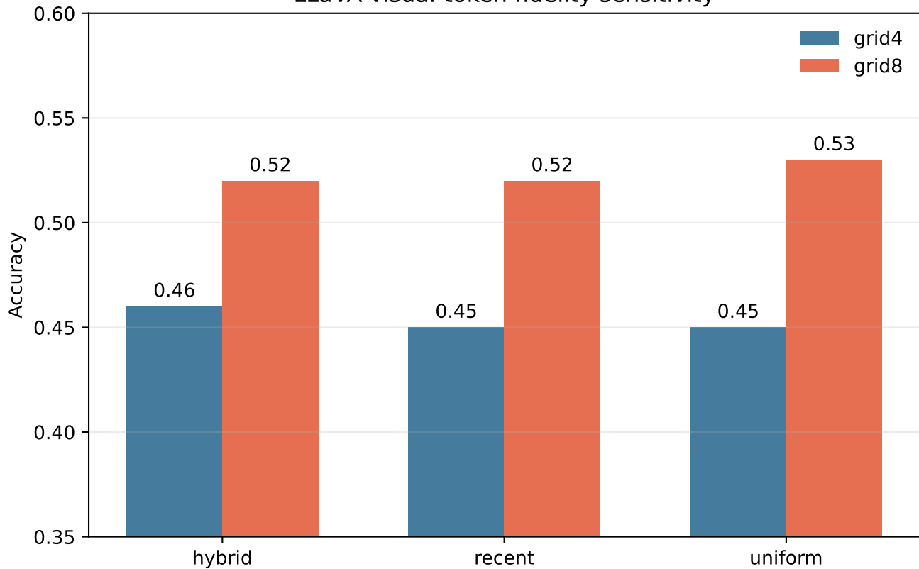
LLaVA visual-token fidelity sensitivity
