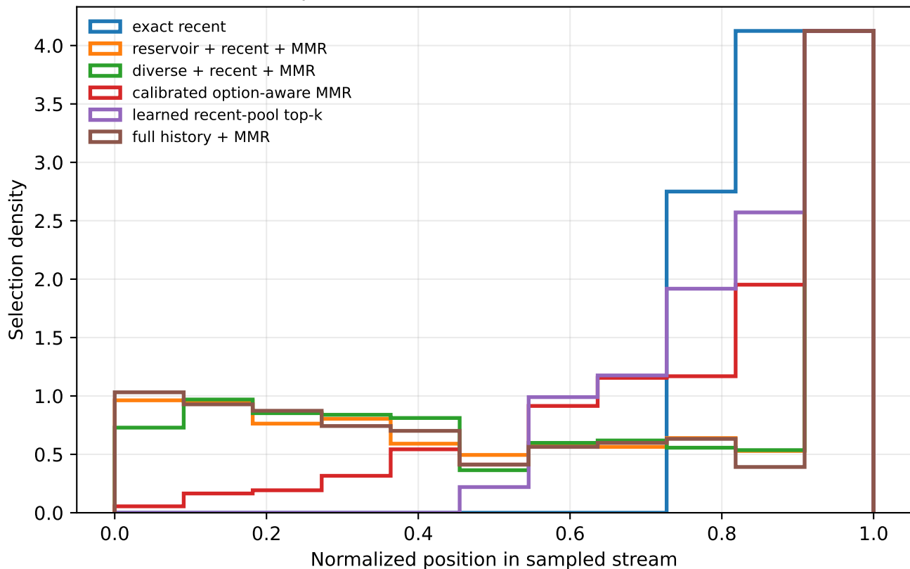
Temporal distribution of selected evidence
