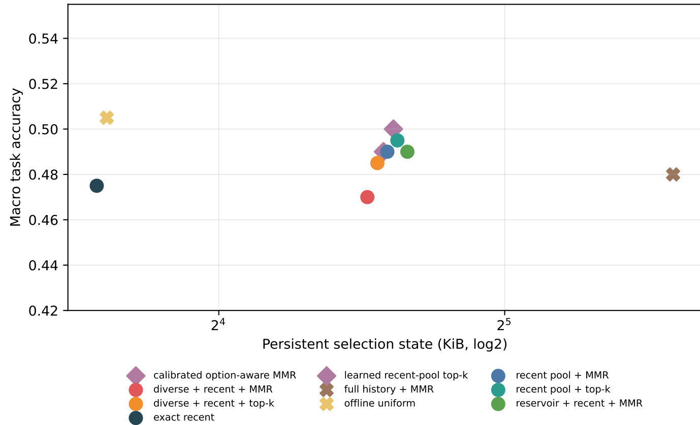
Query-memory accuracy vs persistent state
