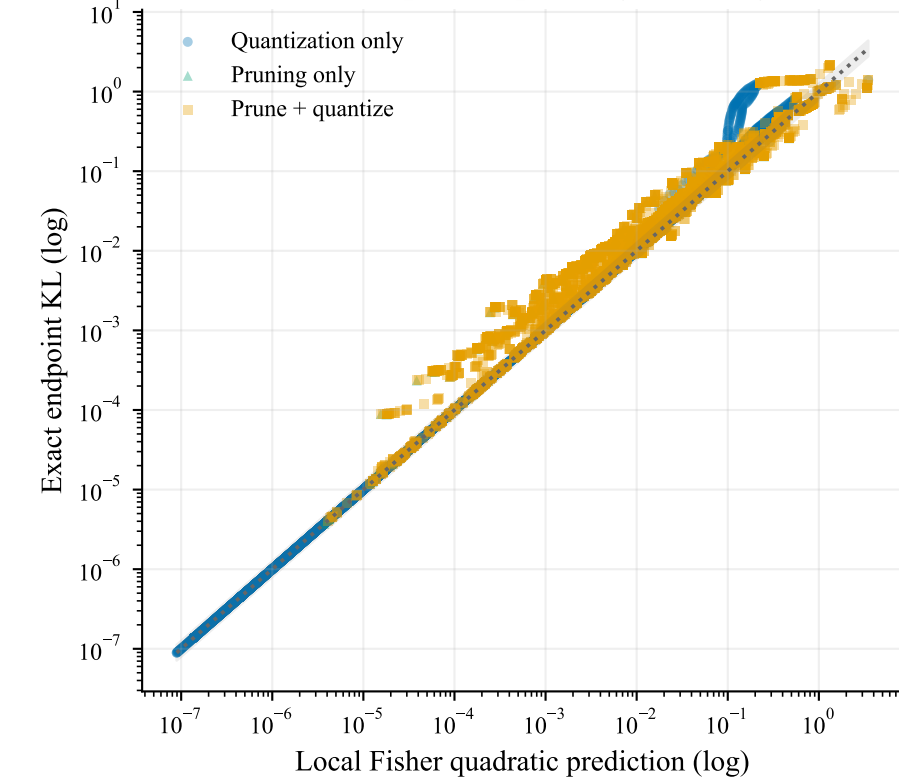
(f) Hessian claims require endpoint Taylor validity
