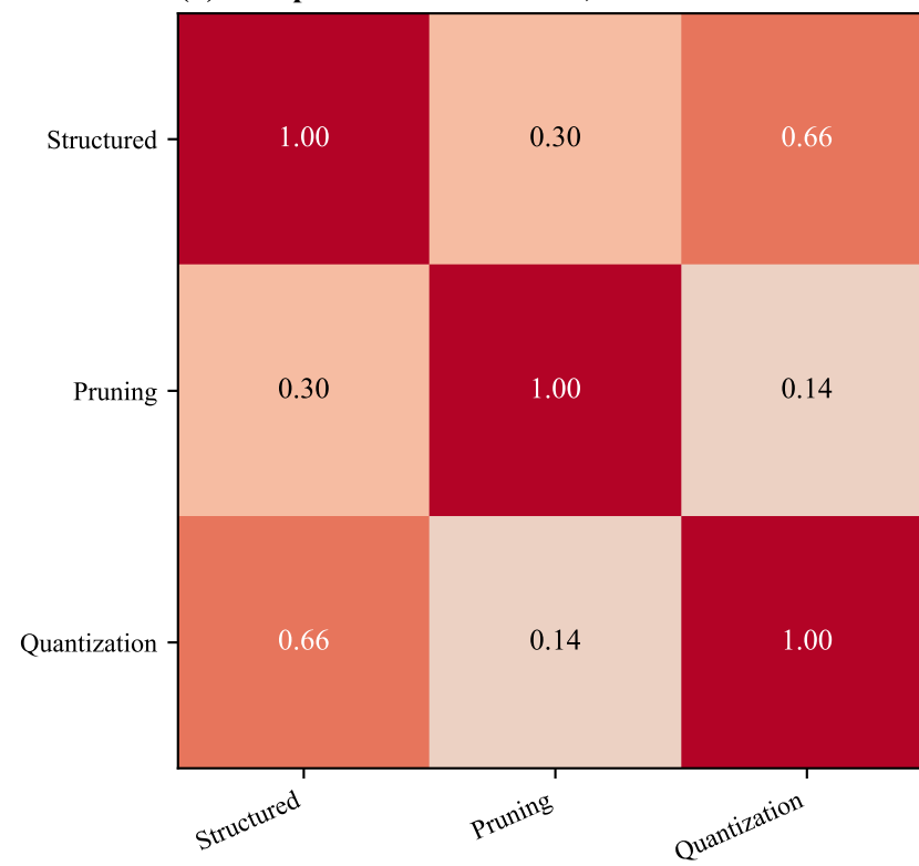
(b) Compression-error cosine, local KL Hessian
