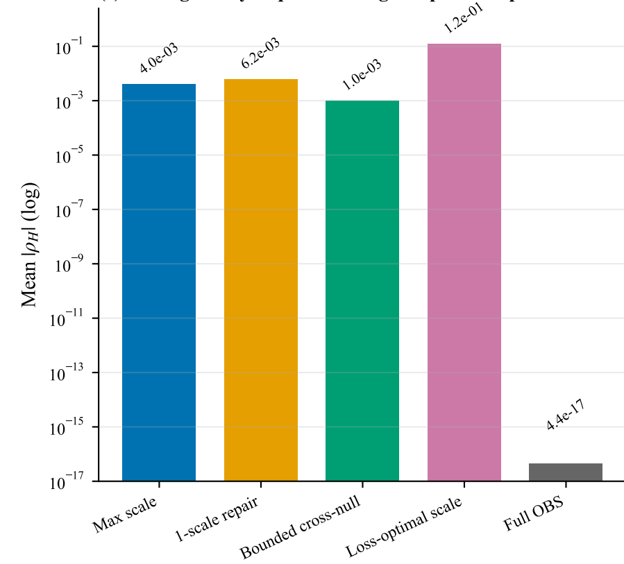
(c) Orthogonality requires the right repair subspace
