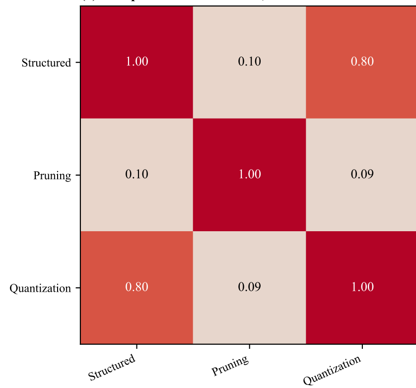
(a) Compression-error cosine, Frobenius metric
