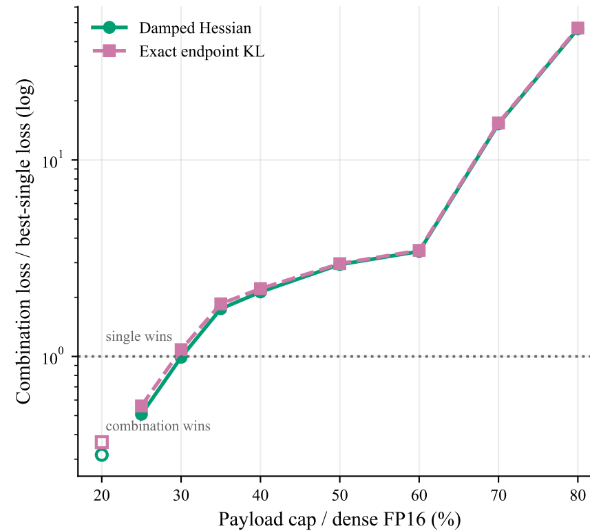
(e) Same codecs: Hessian prediction vs endpoint KL
