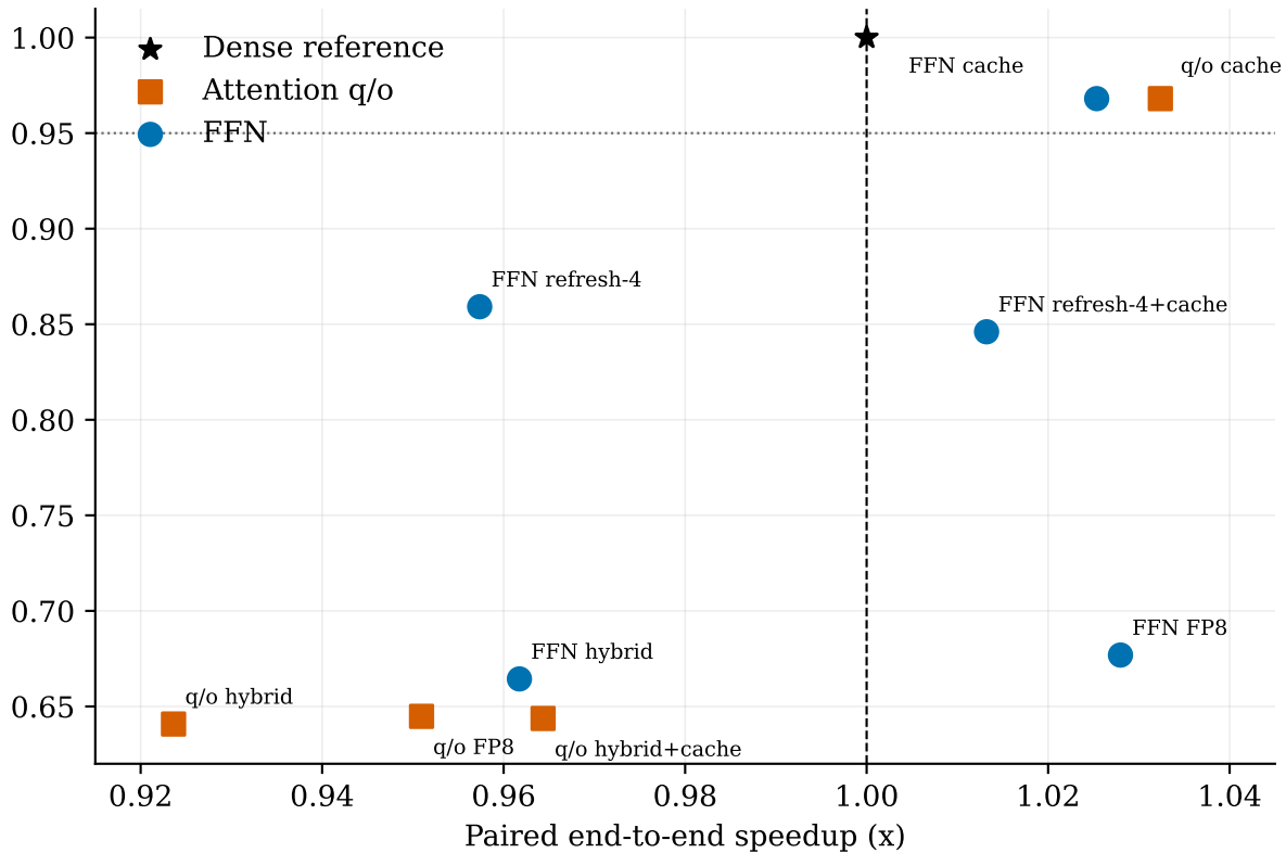
Frame SSIM versus dense
