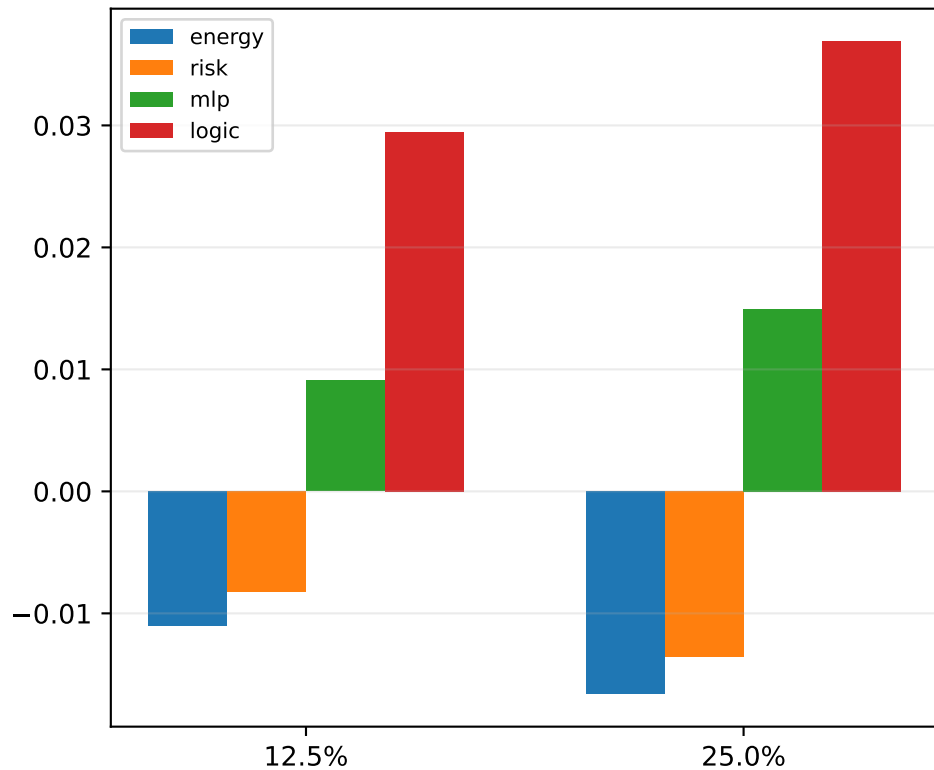
Block Spearman
