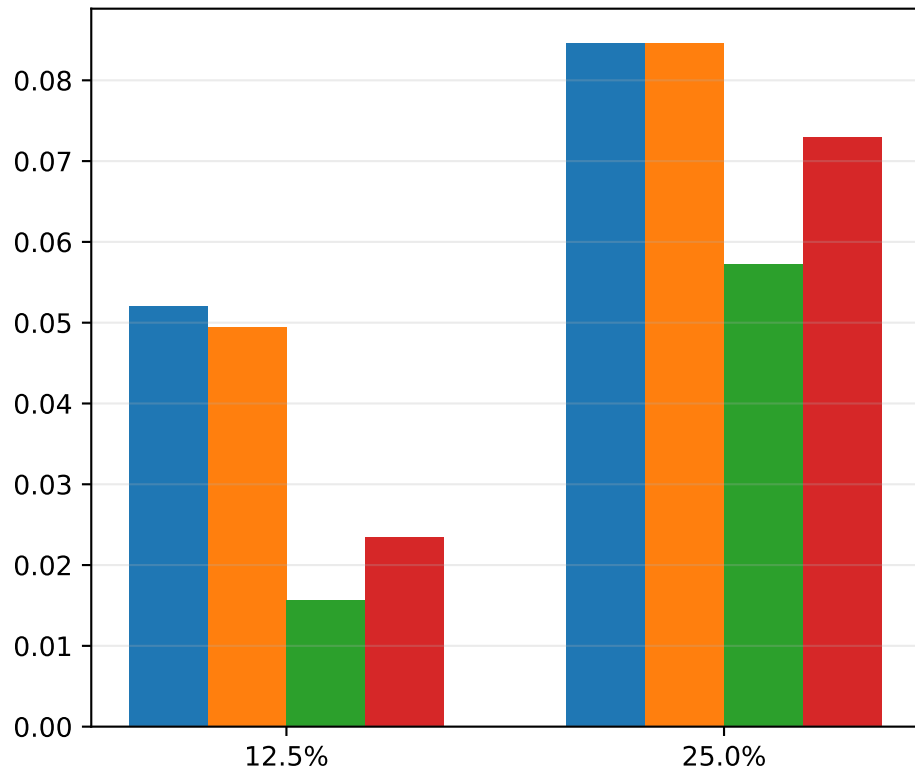
Top-k recall
