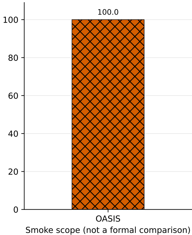
Multiple-choice accuracy (%)
