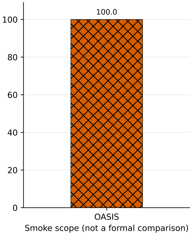
Scored coverage (%)
