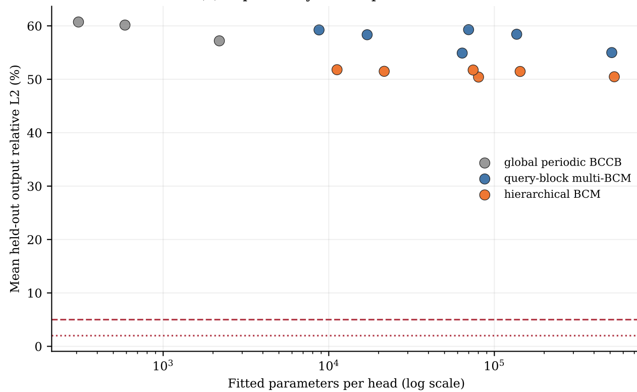
(c) Local tables help only selected heads
