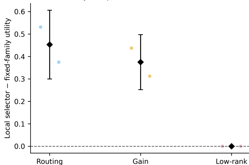
D Fixed-family comparisons
