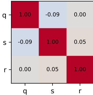
fc2
