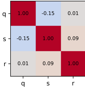
head
