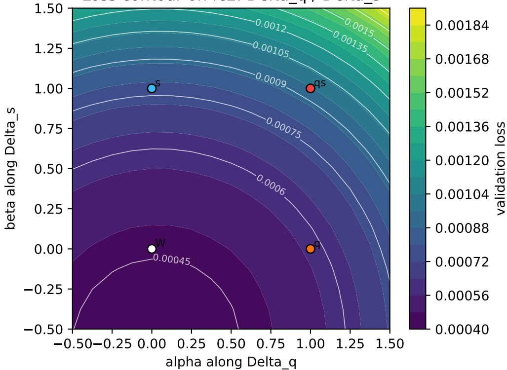
Loss contour on fc2: \Delta_q / \Delta_s
