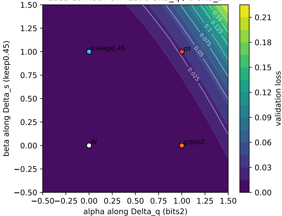
Loss contour on fc2: \Delta_q / \Delta_s
