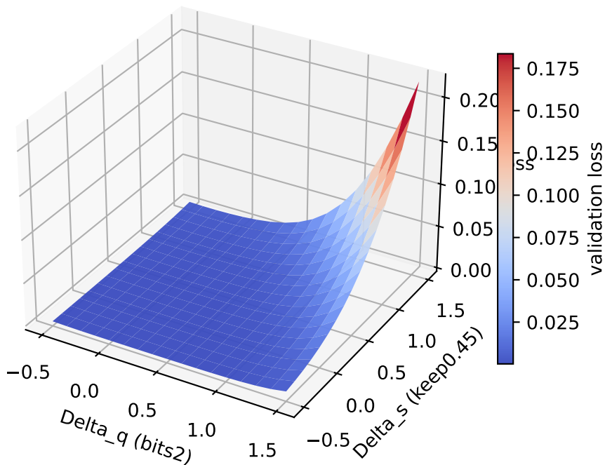
Loss surface on fc2: qs
