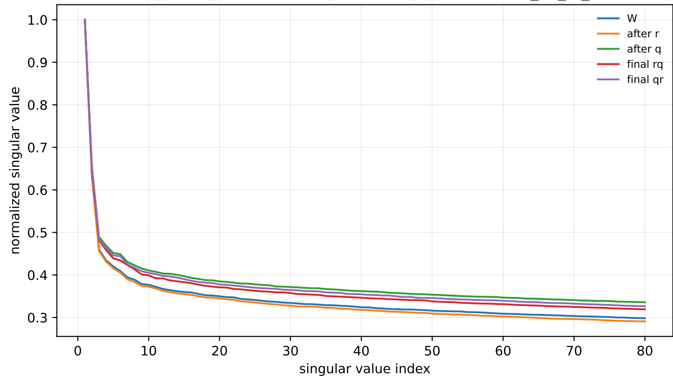
Singular spectrum for largest order gap: L11:dense_4h_to_h
