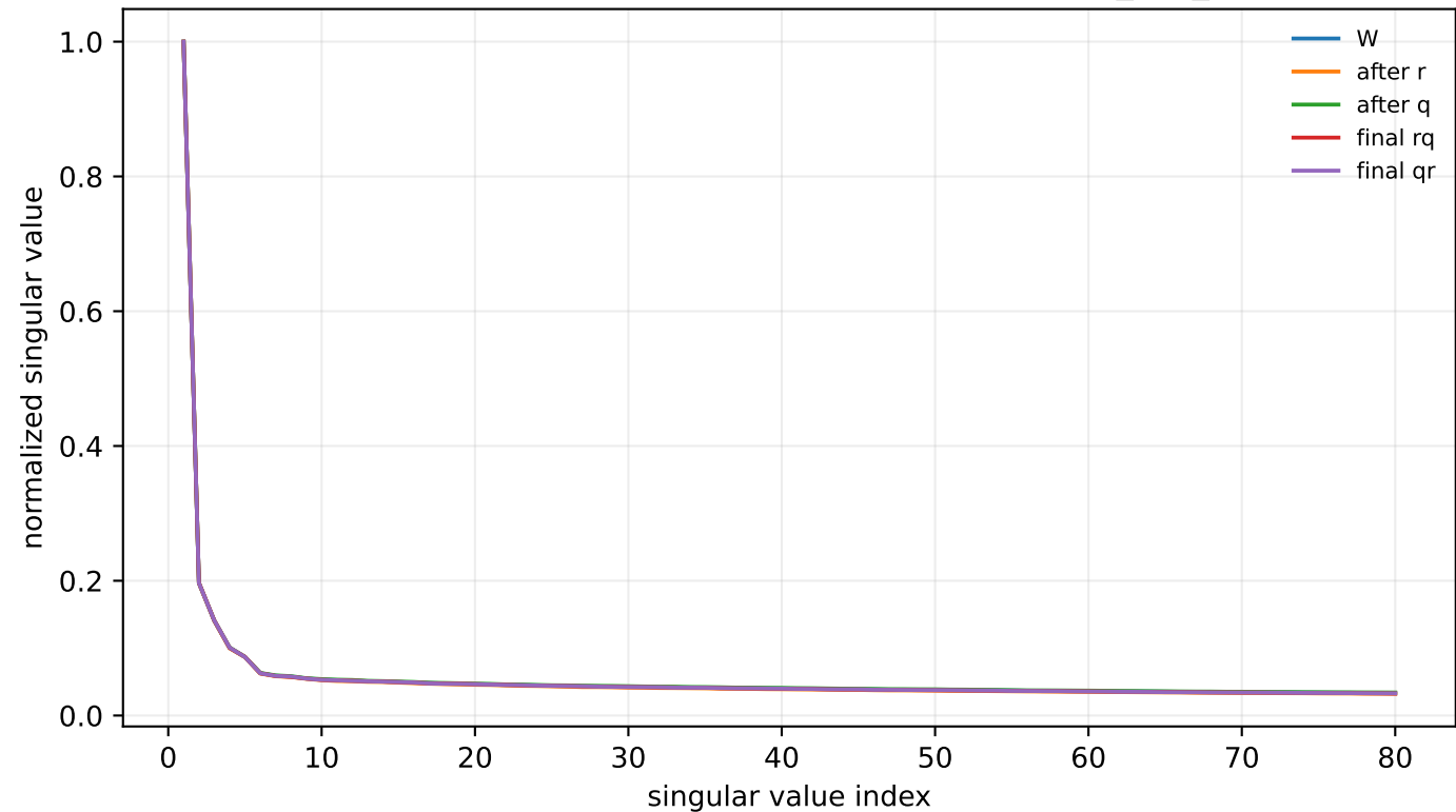
Singular spectrum for largest order gap: L6:query_key_value
