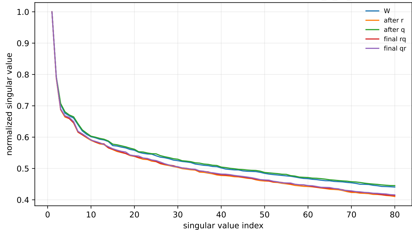
Singular spectrum for largest order gap: L3:dense_h_to_4h
