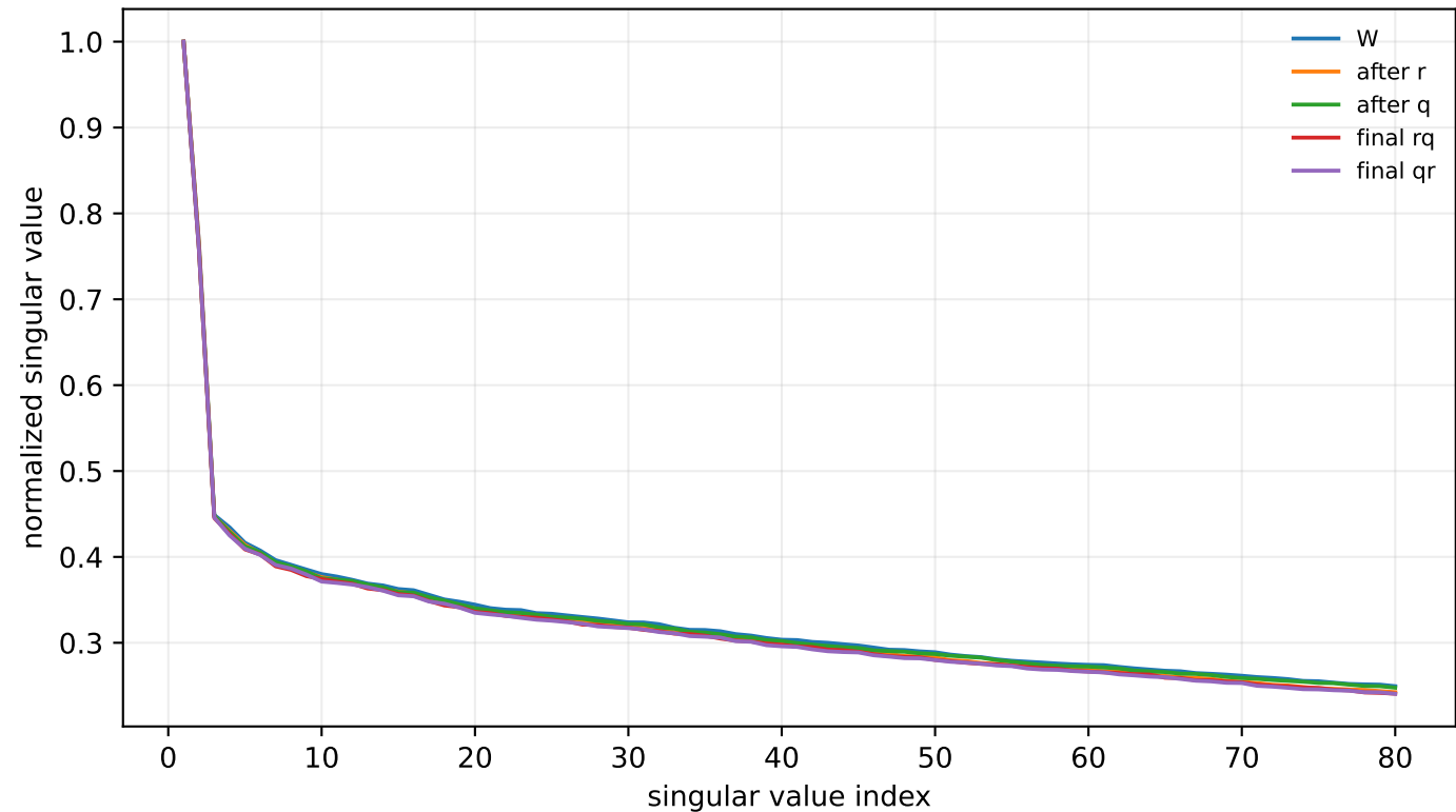
Singular spectrum for largest order gap: L0:dense
