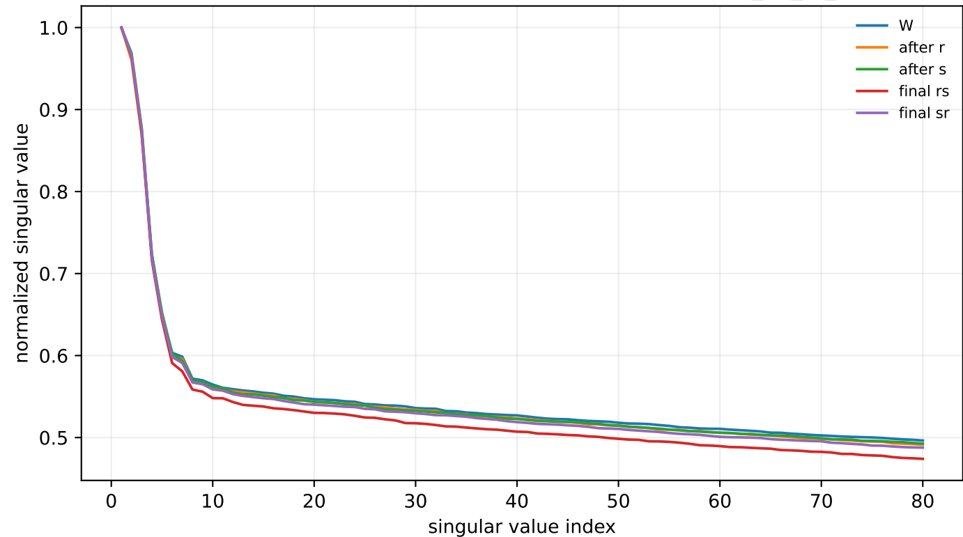
Singular spectrum for largest order gap: L0:dense_4h_to_h
