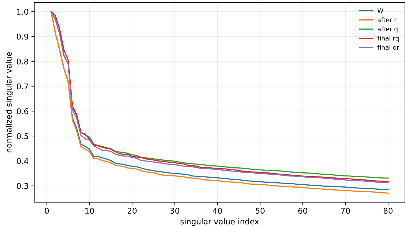
Singular spectrum for largest order gap: L3:dense_4h_to_h
