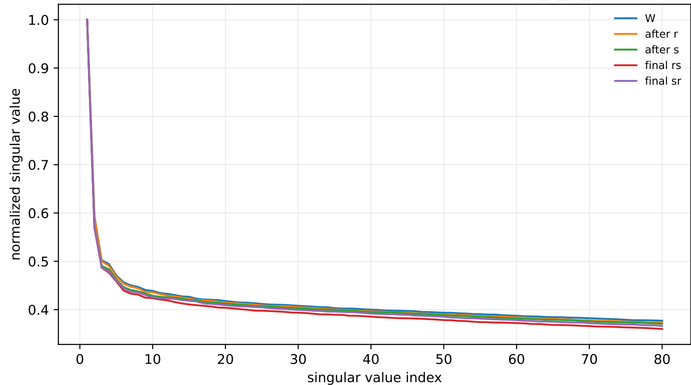
Singular spectrum for largest order gap: L0:dense_h_to_4h
