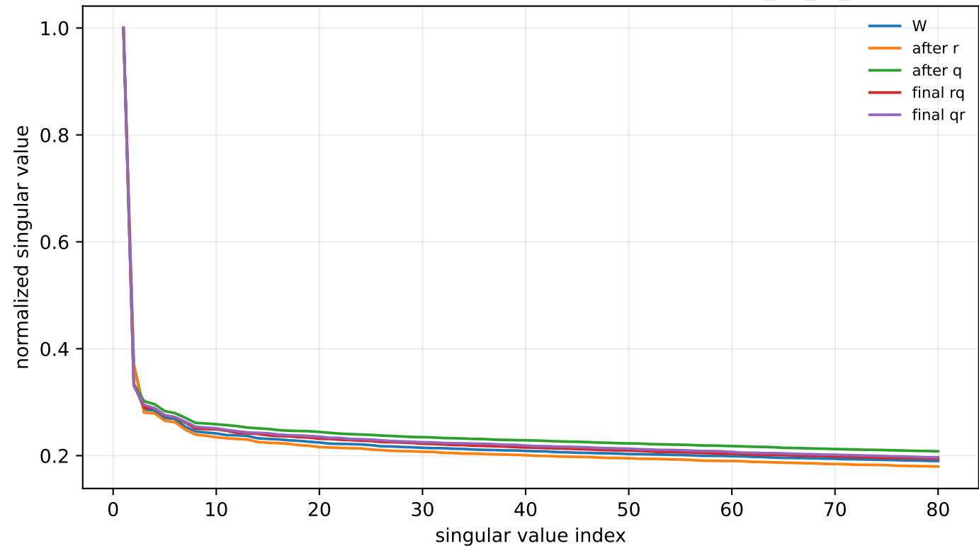
Singular spectrum for largest order gap: L5:dense_4h_to_h
