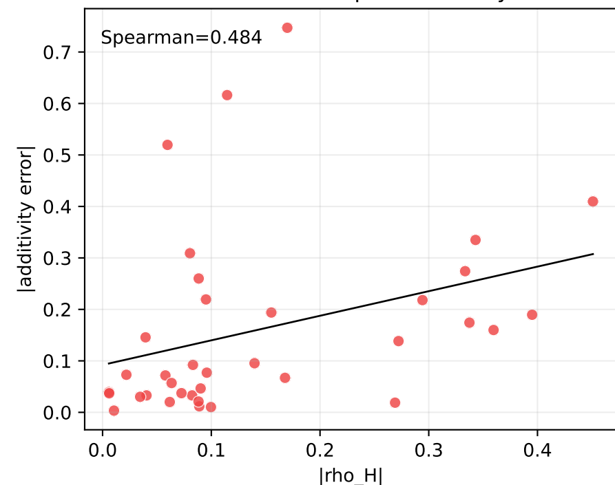
Order-gap explanations
