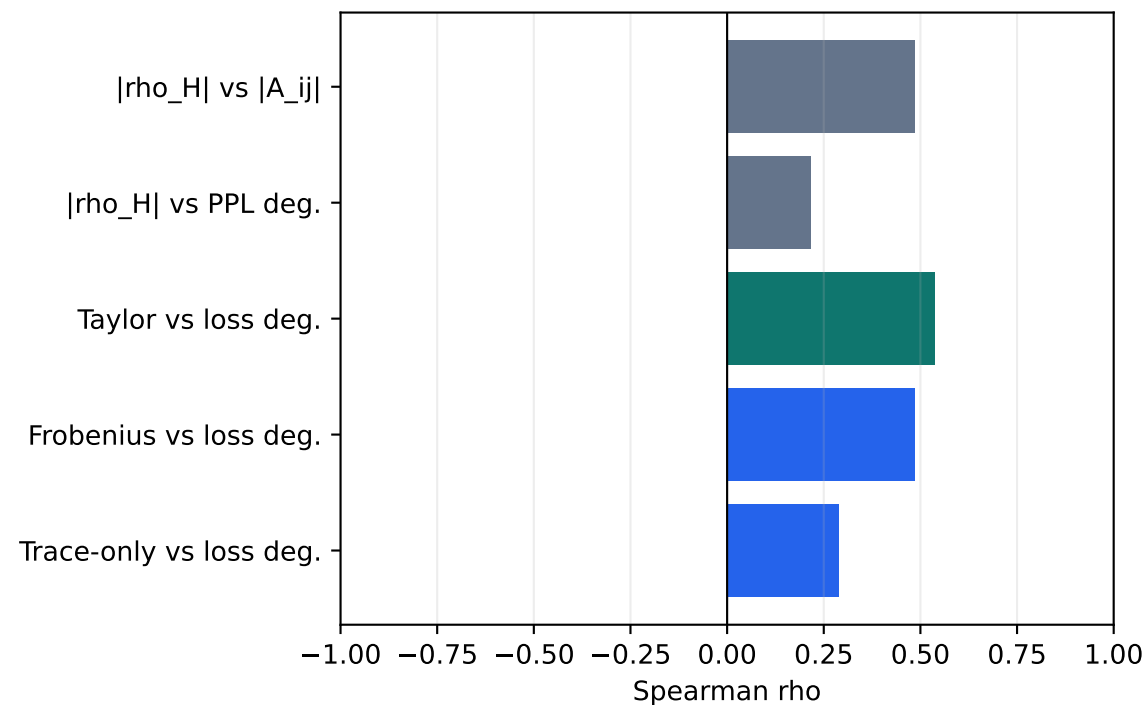
Strategy comparison
