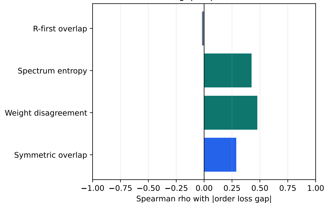
Order-gap explanations
