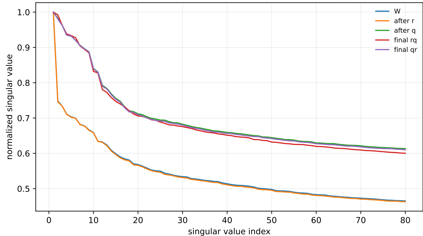
Singular spectrum for largest order gap: L27:down_proj
