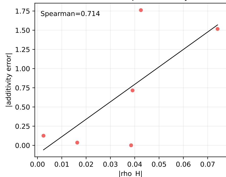
Order-gap explanations
