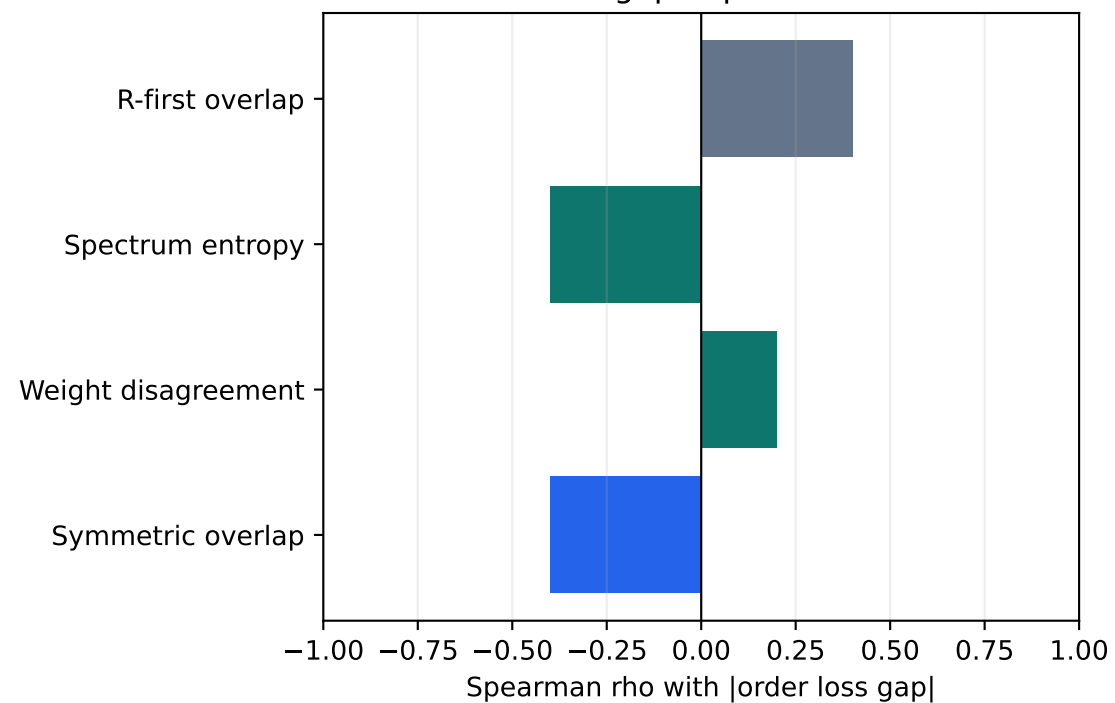
Order-gap explanations
