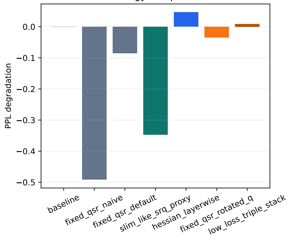
Strategy comparison
