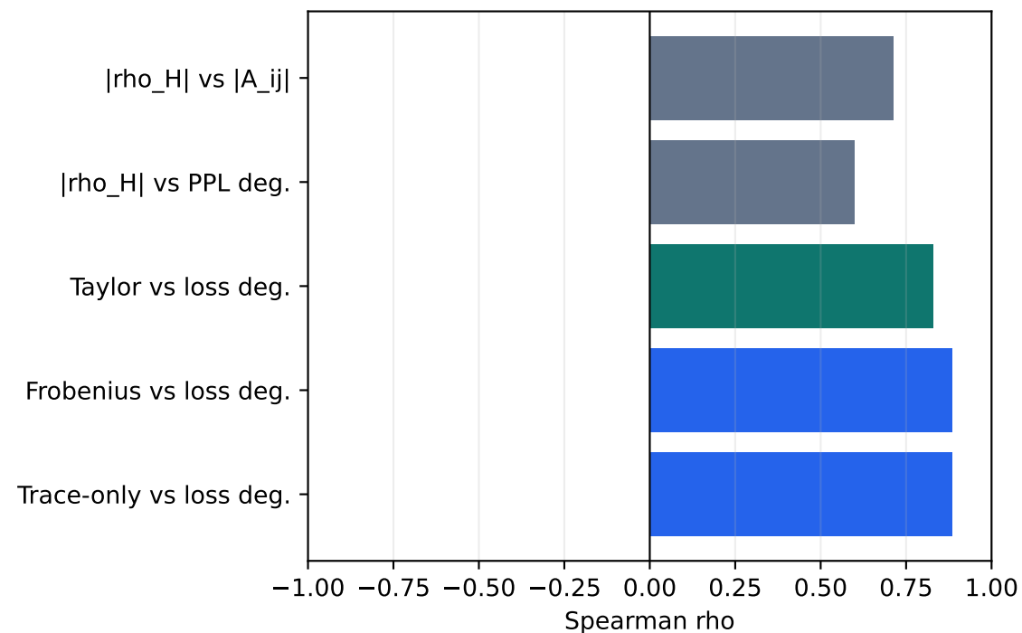
Strategy comparison
