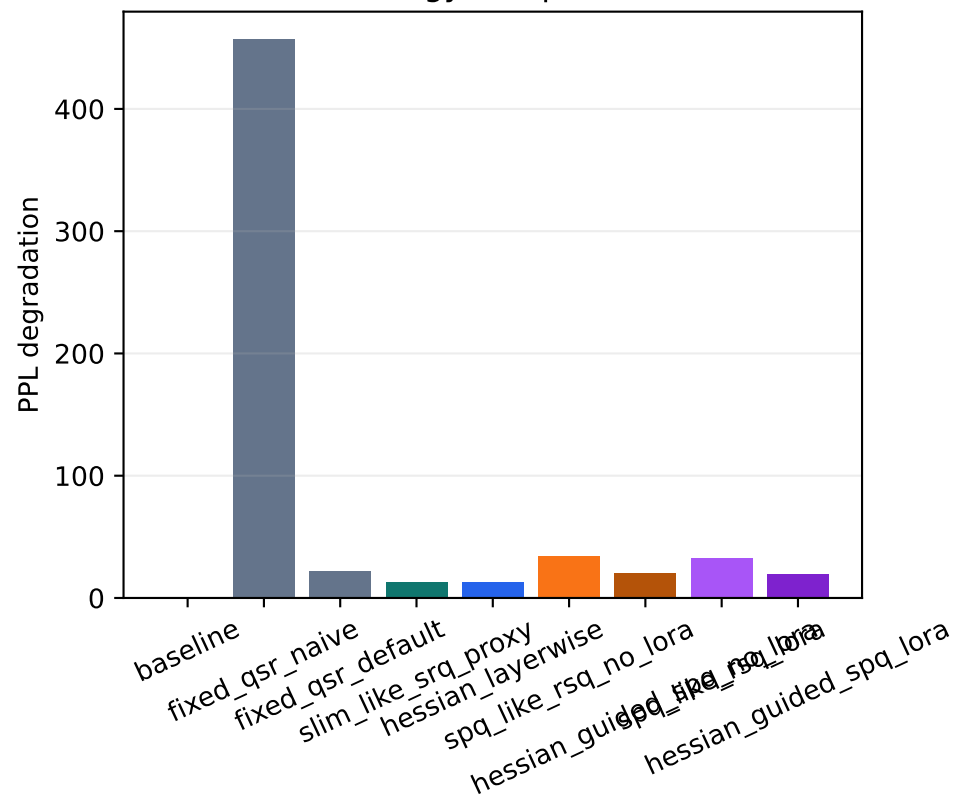
Strategy comparison
