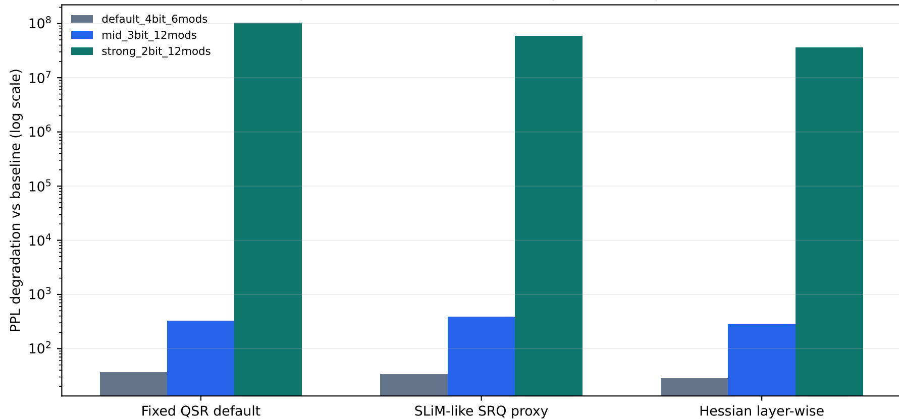
Layer-wise selection vs fixed compression recipes
