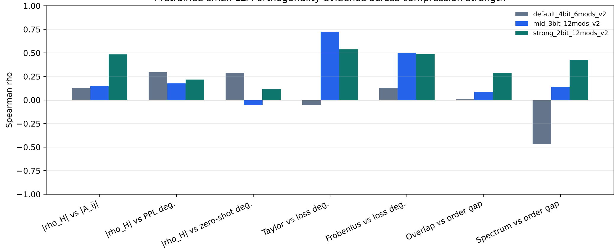
Pretrained small-LLM orthogonality evidence across compression strength
