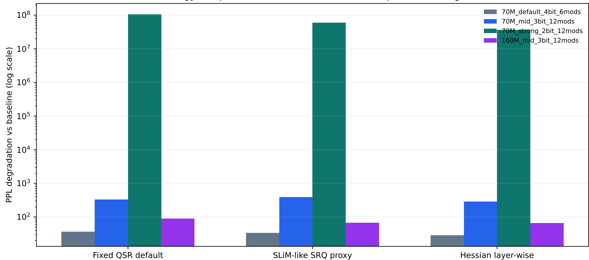
Strategy comparison across model size and compression strength
