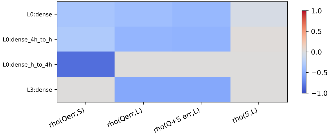
Conditional Hessian overlap for selected residual recipe
