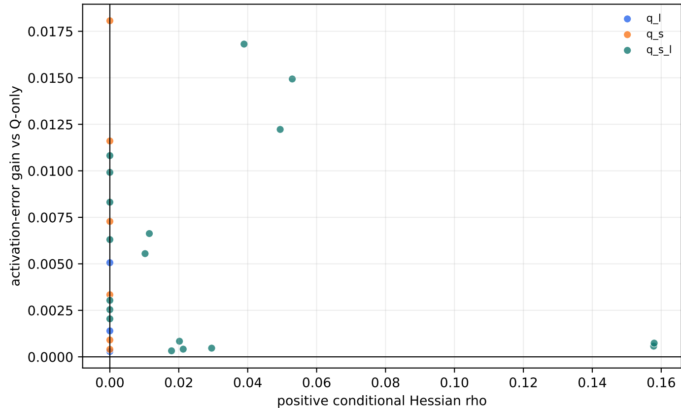
Residual structure benefit vs overlap
