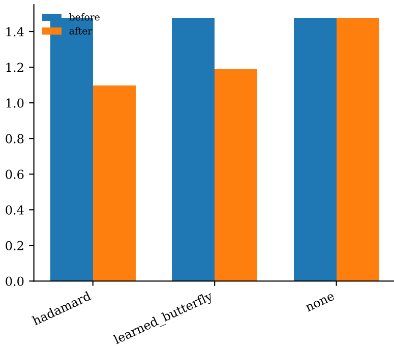
Input-channel max/median
