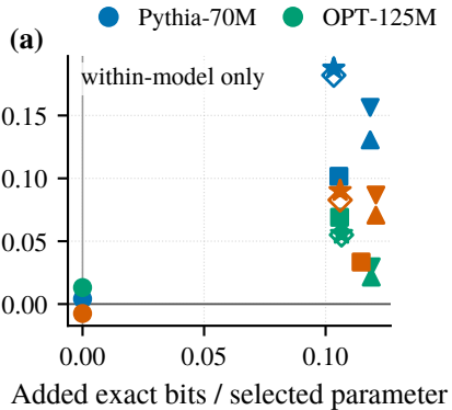
NLL recovery from Q (nats/token)
