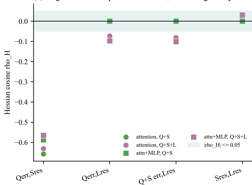
(c) Negative rho is repair cancellation, not orthogonality
