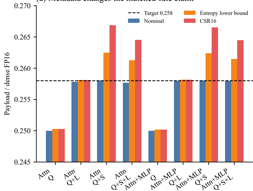
(a) Metadata changes the matched-rate claim
