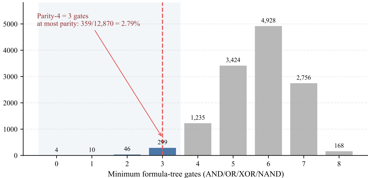
Balanced 4-input functions
